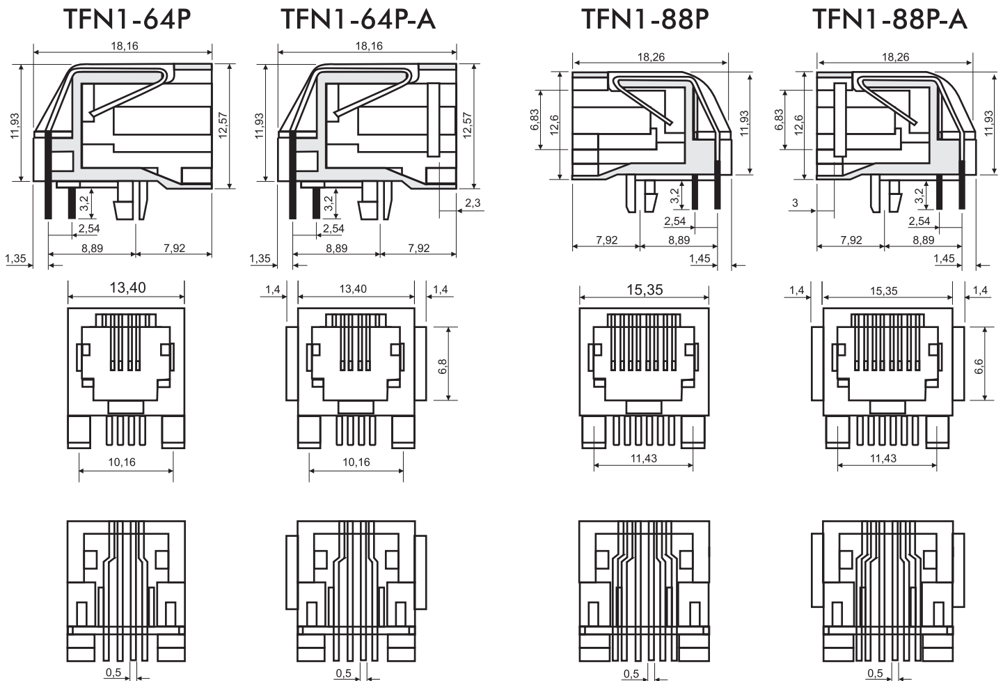
Diagrama PCI / Printed circuit layout
