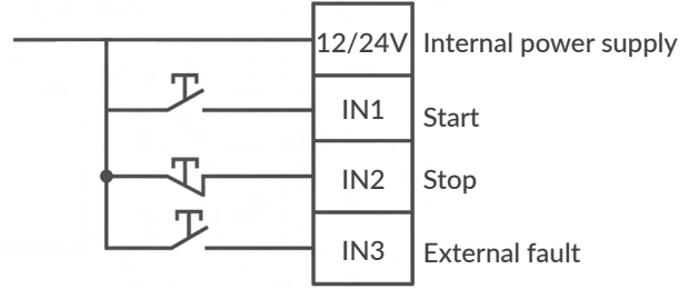
Three-wire system
