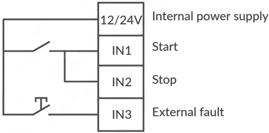
Two-wire system
