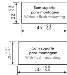
Corte do painel Panel cut out
