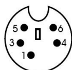
Vista frontal Mini-DIN macho
